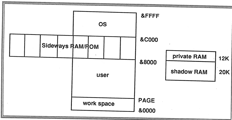
Figure 3. System with sideways and shadow RAM
