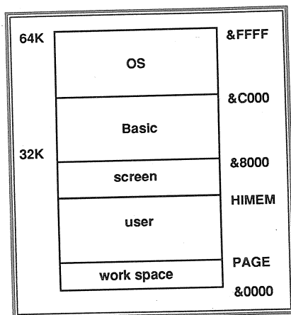
Figure 2. Basic RAM/ROM layout
