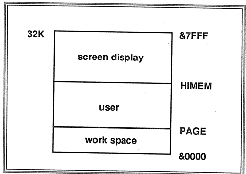
Figure 1. Basic RAM allocation
